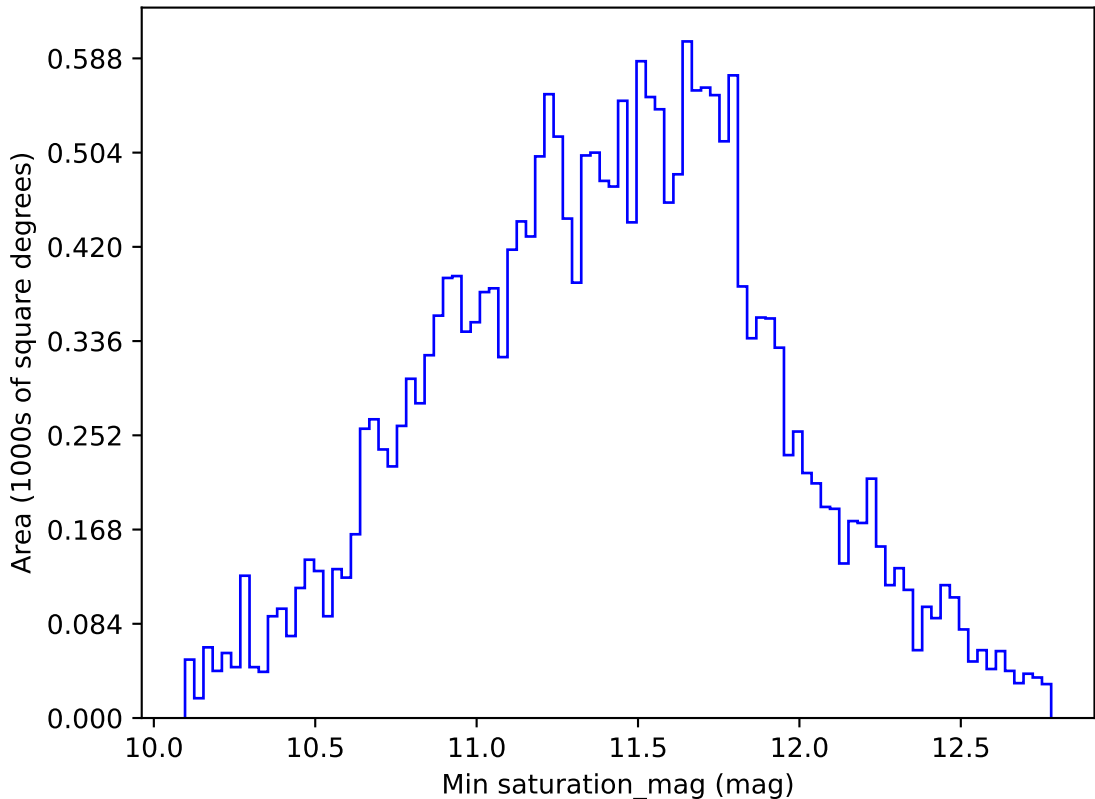
too_elab_r64_d2_giz_v3.4_10yrs All sky u band: Min saturation_mag
