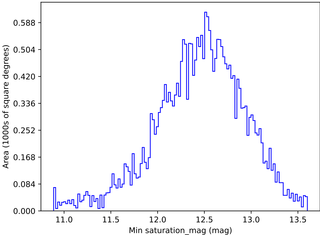
too_elab_r64_d2_giz_v3.4_10yrs All sky i band: Min saturation_mag
