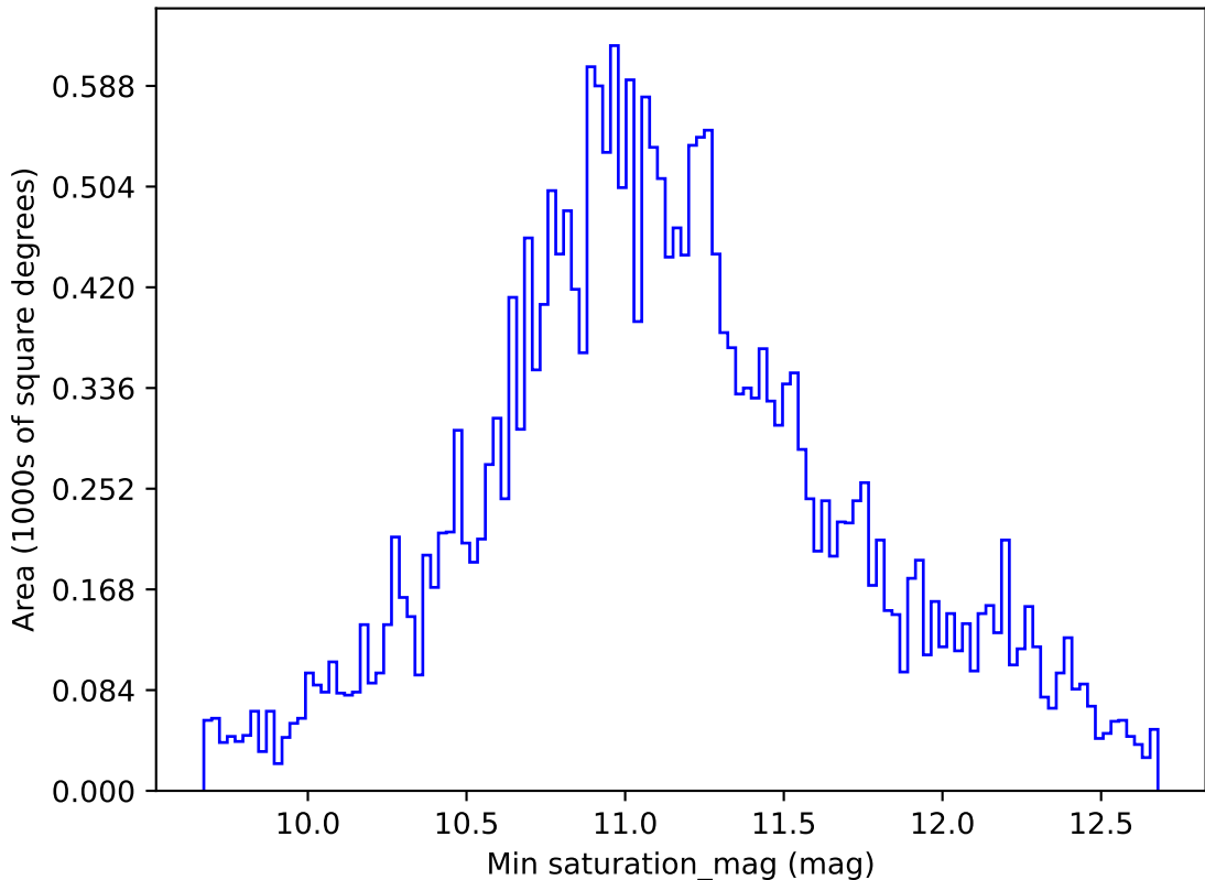
too_elab_r64_d2_giz_v3.4_10yrs All sky all bands: Min saturation_mag
