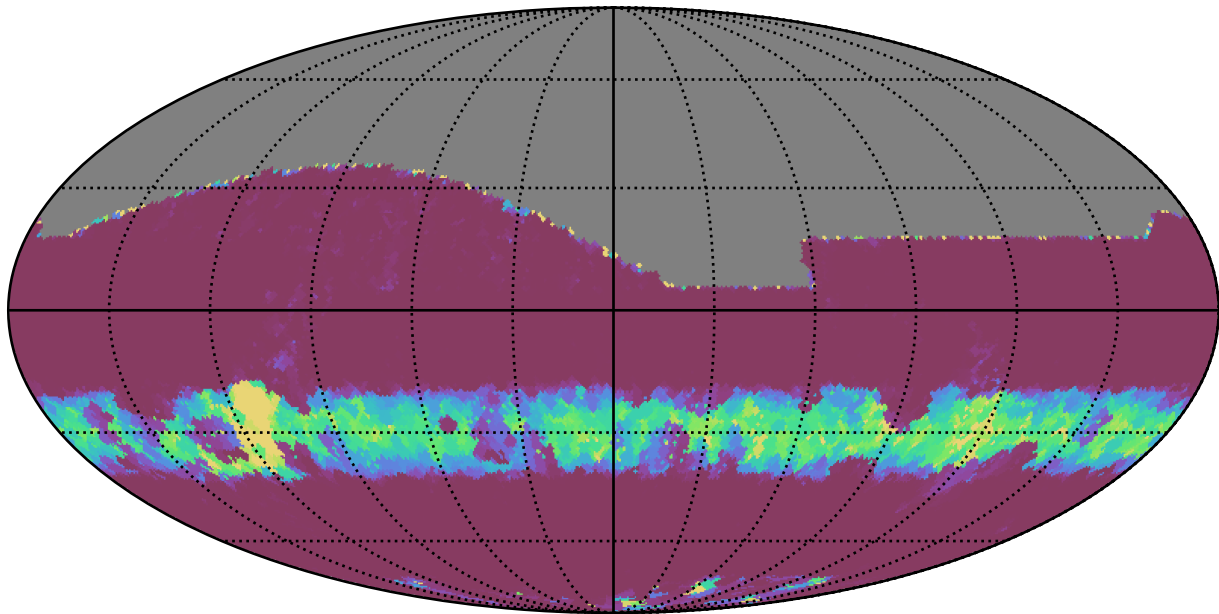
too_elab_r64_d2_giz_v3.4_10yrs All sky z band: Min normairmass
