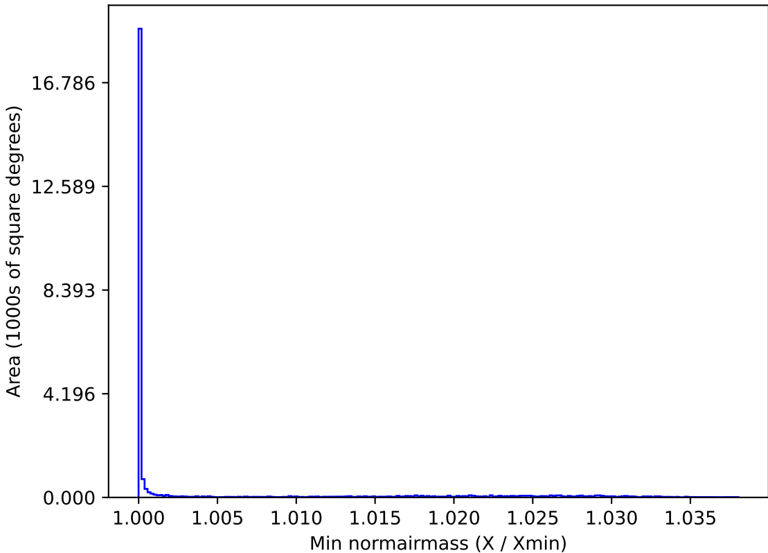
too_elab_r64_d2_giz_v3.4_10yrs All sky r band: Min normairmass
