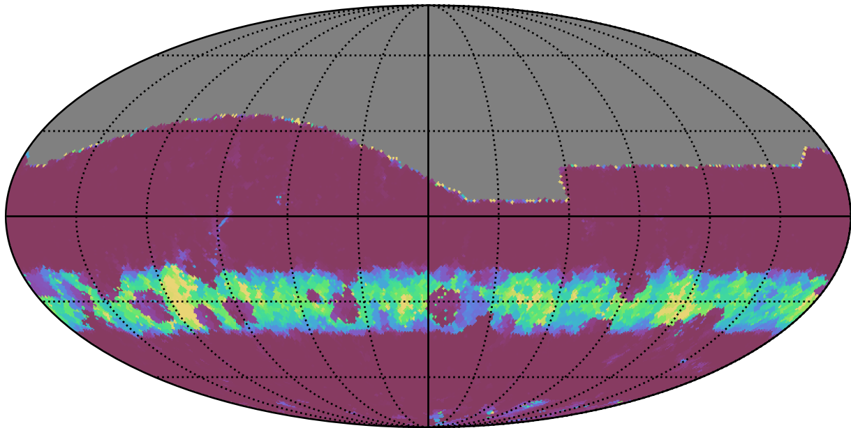
too_elab_r64_d2_giz_v3.4_10yrs All sky g band: Min normairmass
