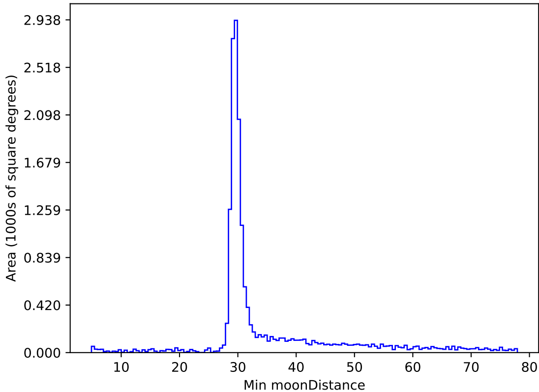
too_elab_r64_d2_giz_v3.4_10yrs WFD z band: Min moonDistance
