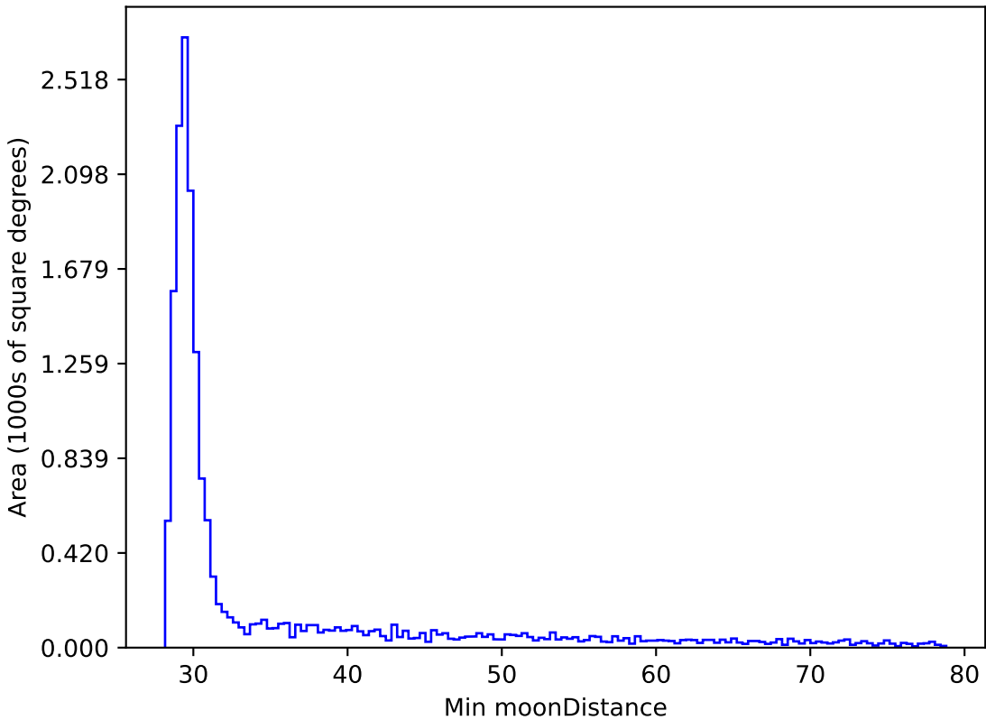
too_elab_r64_d2_giz_v3.4_10yrs WFD y band: Min moonDistance
