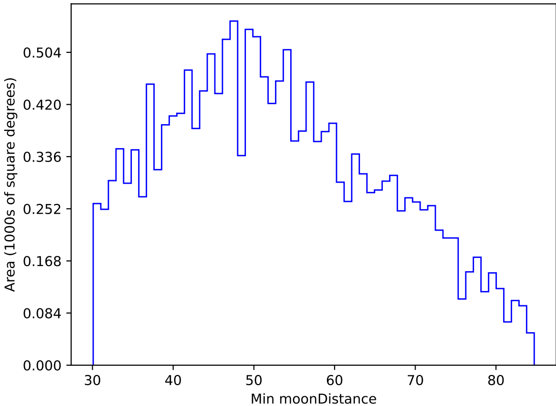
too_elab_r64_d2_giz_v3.4_10yrs WFD u band: Min moonDistance
