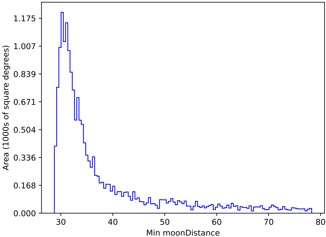
too_elab_r64_d2_giz_v3.4_10yrs WFD r band: Min moonDistance
