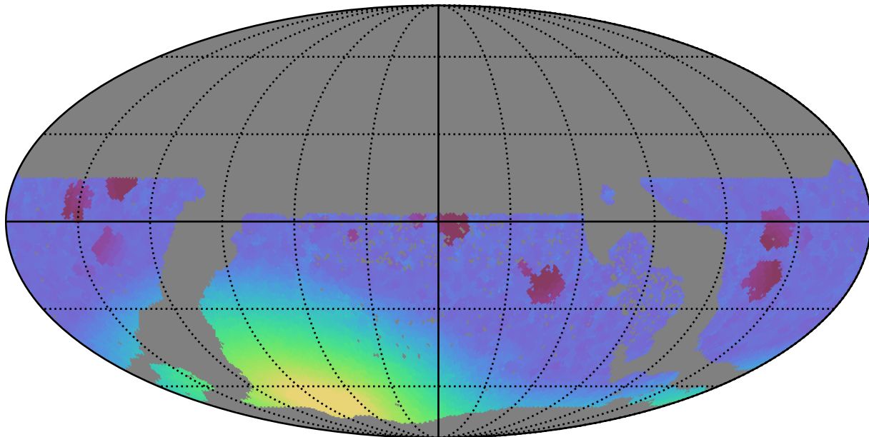
too_elab_r64_d2_giz_v3.4_10yrs WFD i band: Min moonDistance
