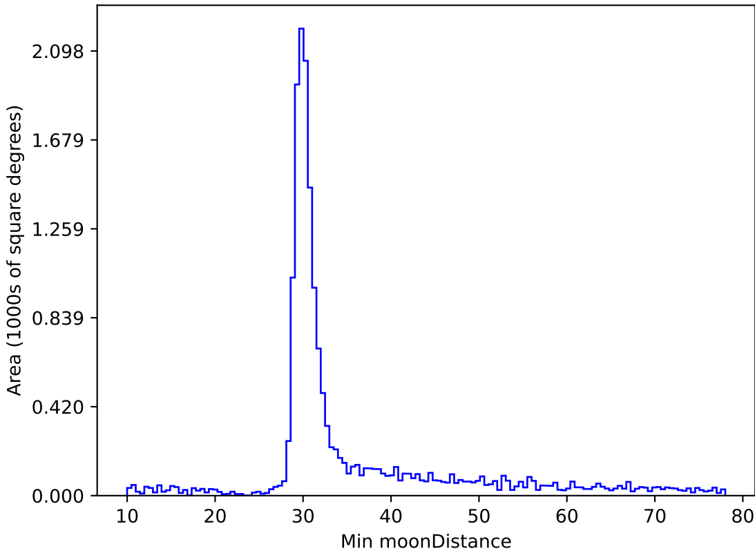
too_elab_r64_d2_giz_v3.4_10yrs WFD i band: Min moonDistance
