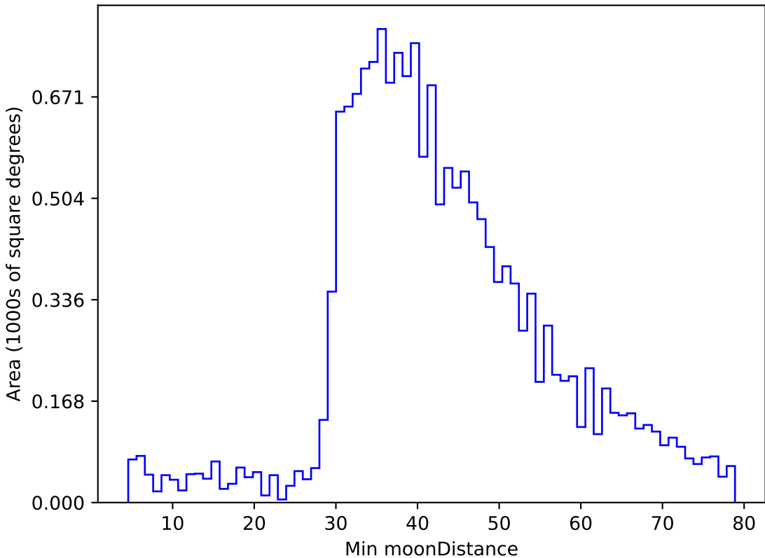
too_elab_r64_d2_giz_v3.4_10yrs WFD g band: Min moonDistance
