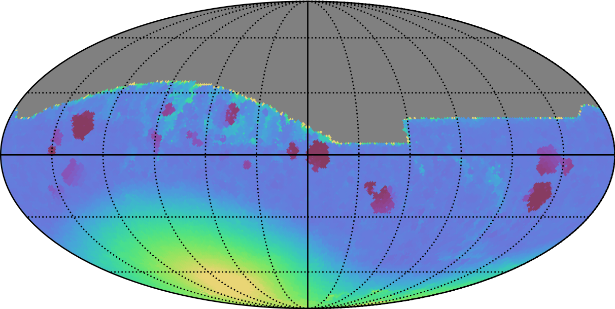
too_elab_r64_d2_giz_v3.4_10yrs All sky z band: Min moonDistance
