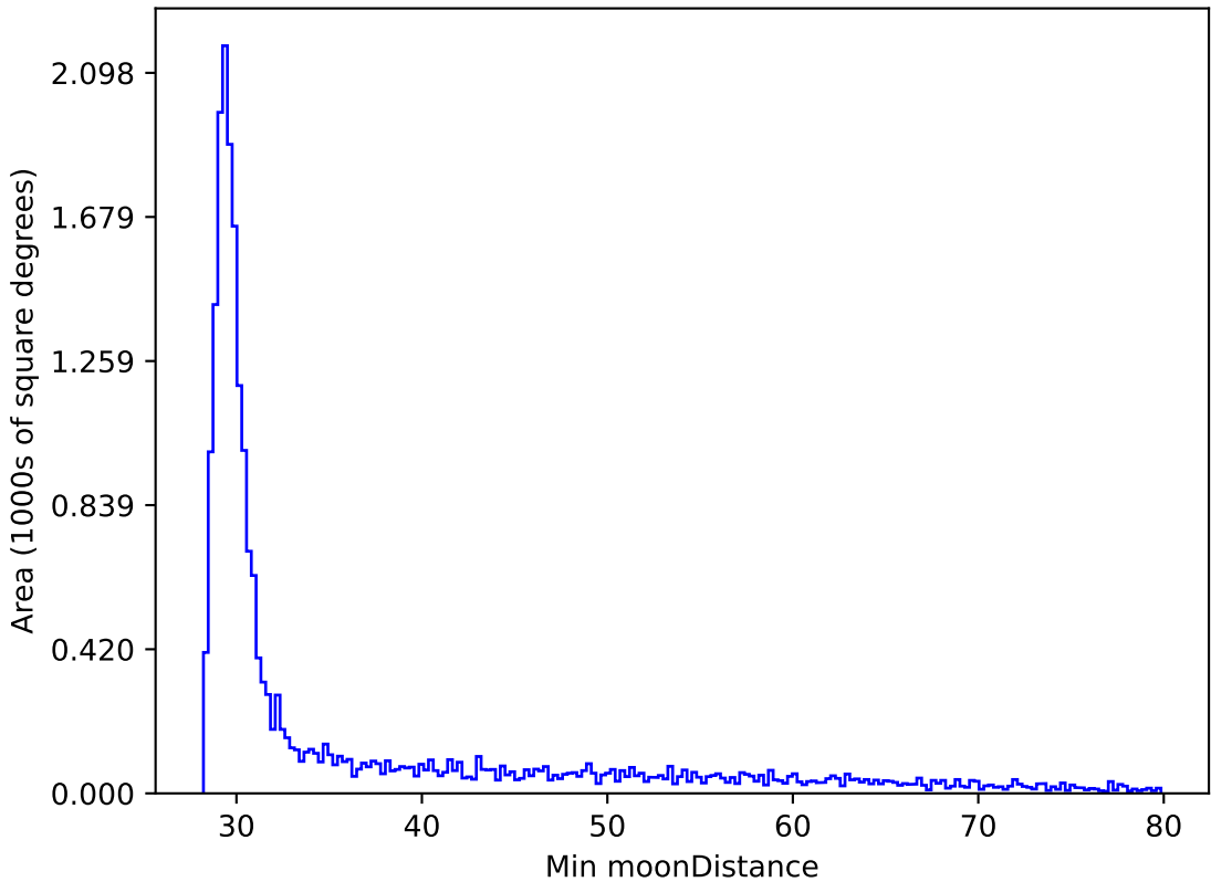
too_elab_r64_d2_giz_v3.4_10yrs All sky y band: Min moonDistance
