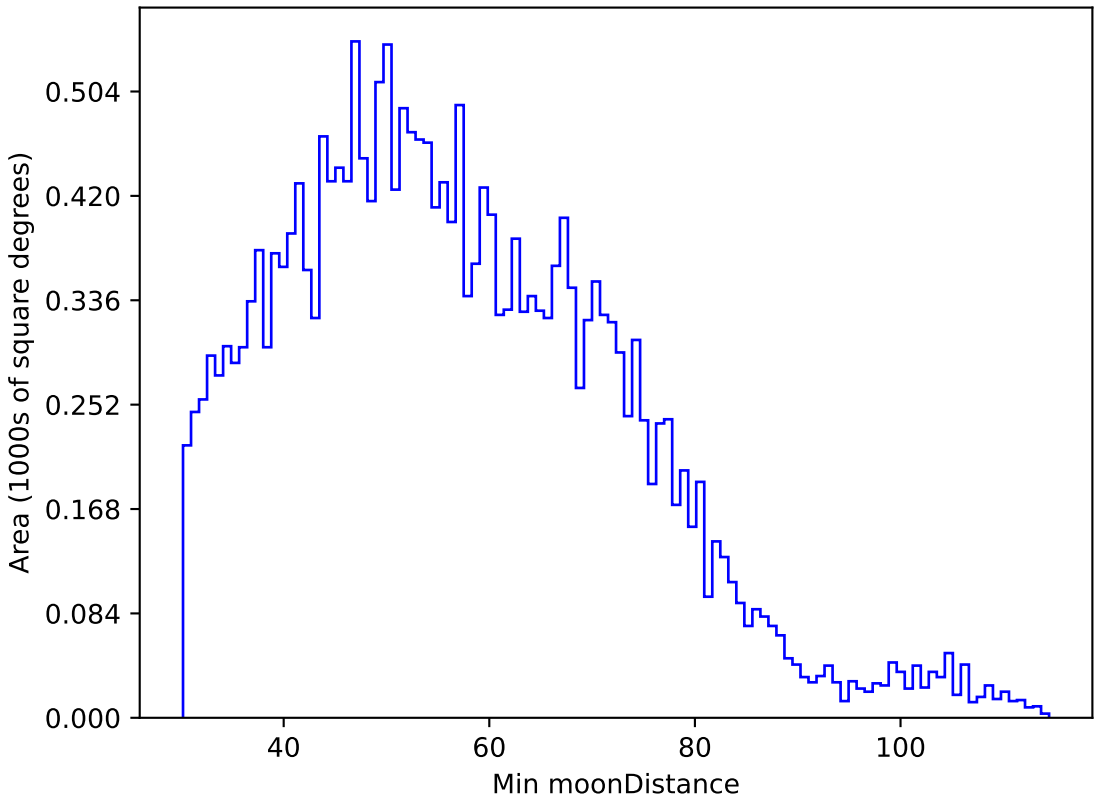
too_elab_r64_d2_giz_v3.4_10yrs All sky u band: Min moonDistance
