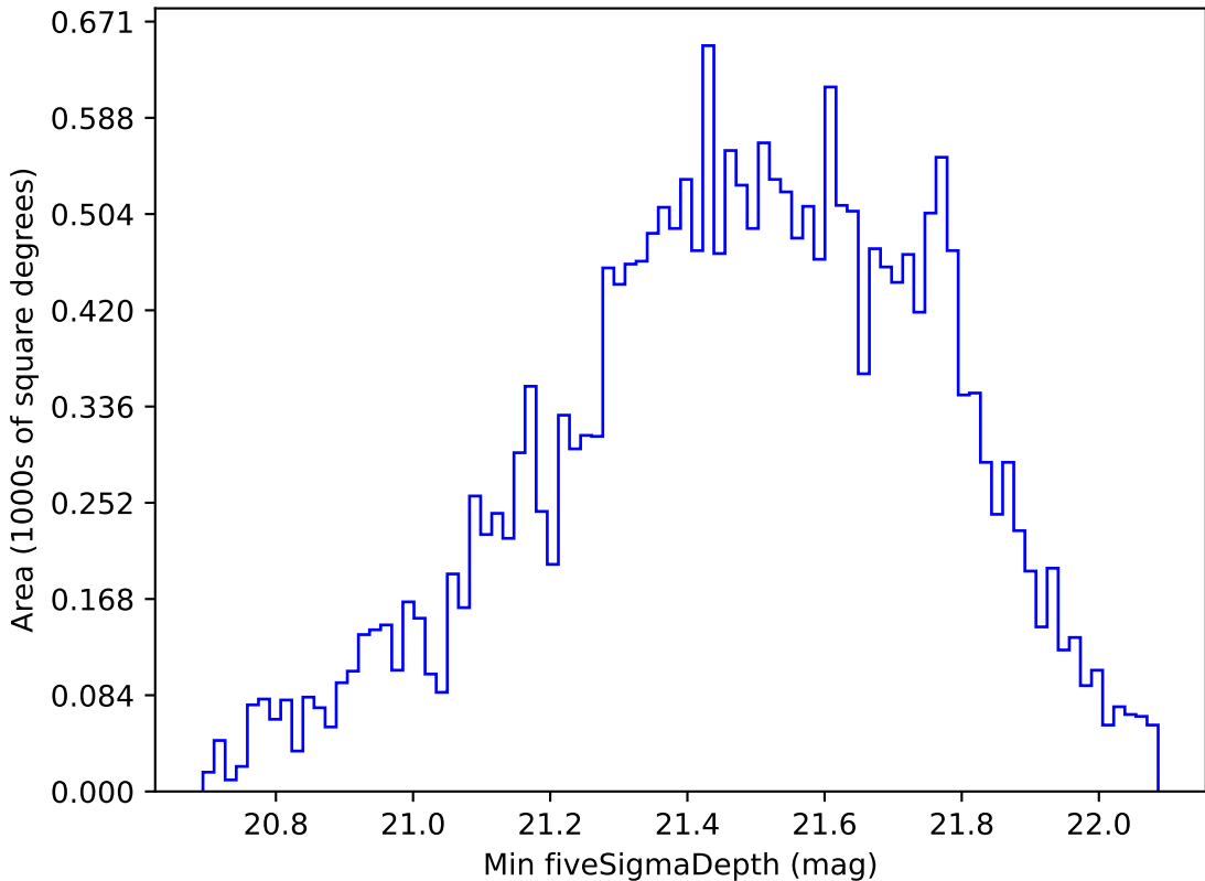
too_elab_r64_d2_giz_v3.4_10yrs Yr 1 y band: Min fiveSigmaDepth
