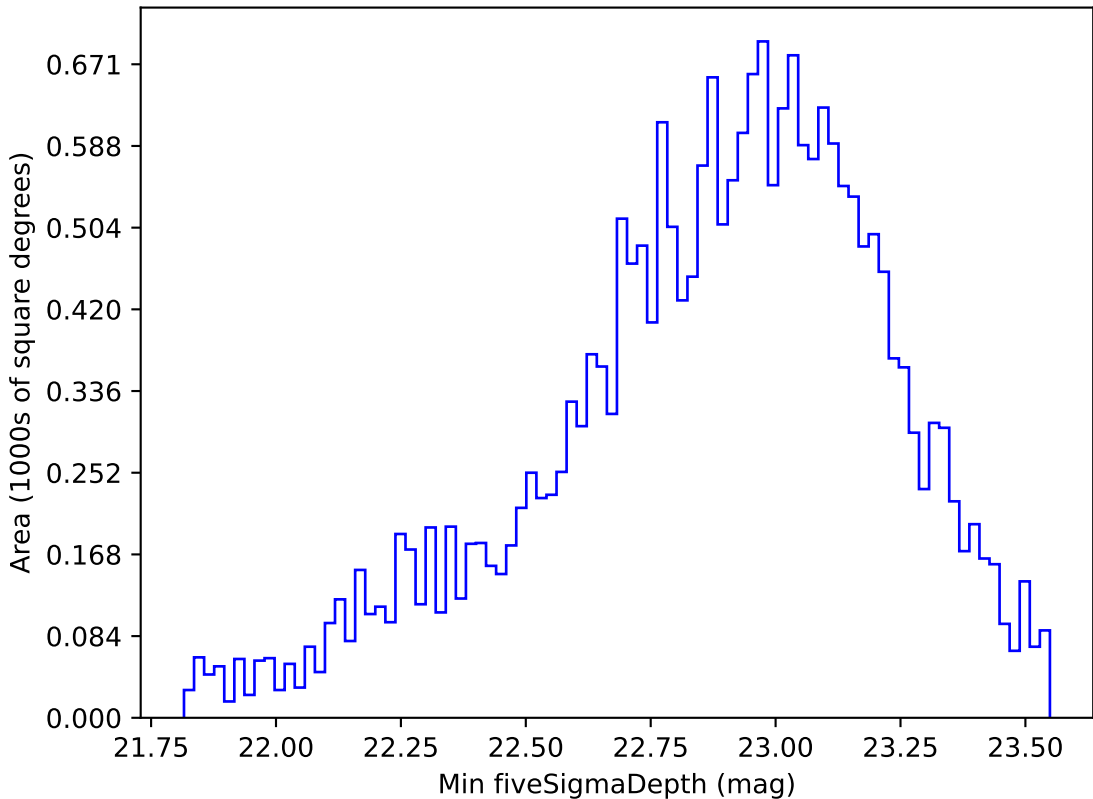
too_elab_r64_d2_giz_v3.4_10yrs Yr 1 u band: Min fiveSigmaDepth
