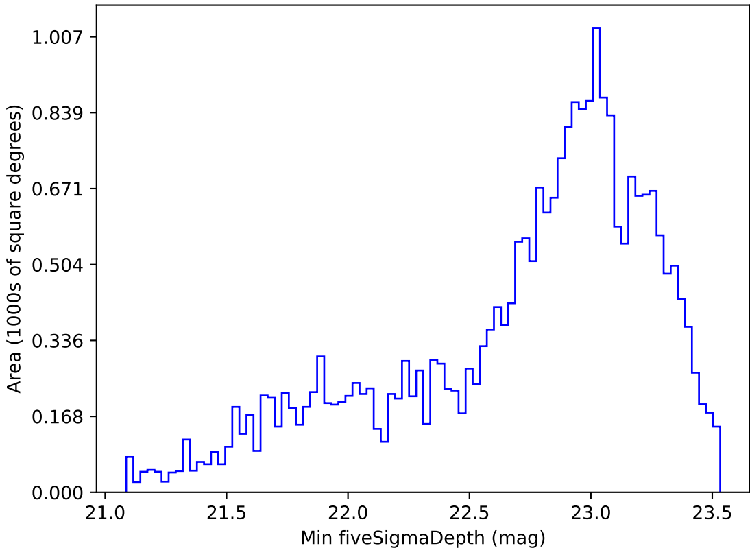
too_elab_r64_d2_giz_v3.4_10yrs Yr 1 i band: Min fiveSigmaDepth
