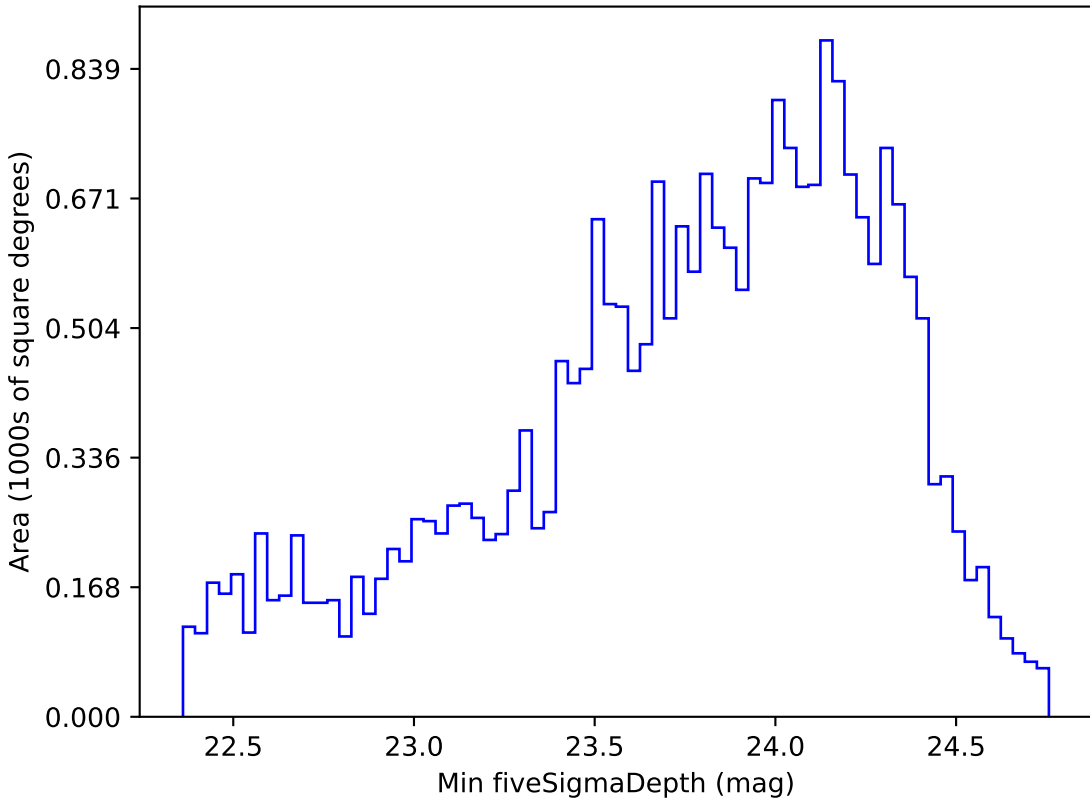
too_elab_r64_d2_giz_v3.4_10yrs Yr 1 g band: Min fiveSigmaDepth
