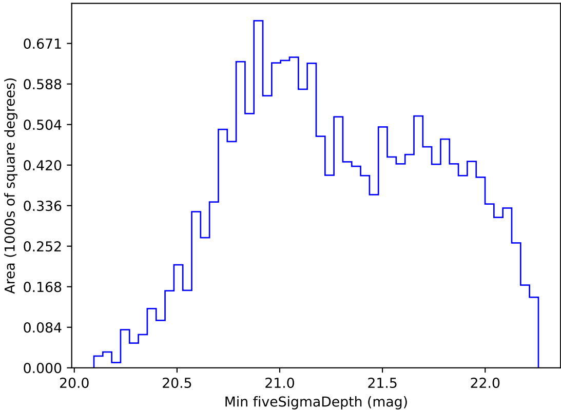
too_elab_r64_d2_giz_v3.4_10yrs WFD z band: Min fiveSigmaDepth
