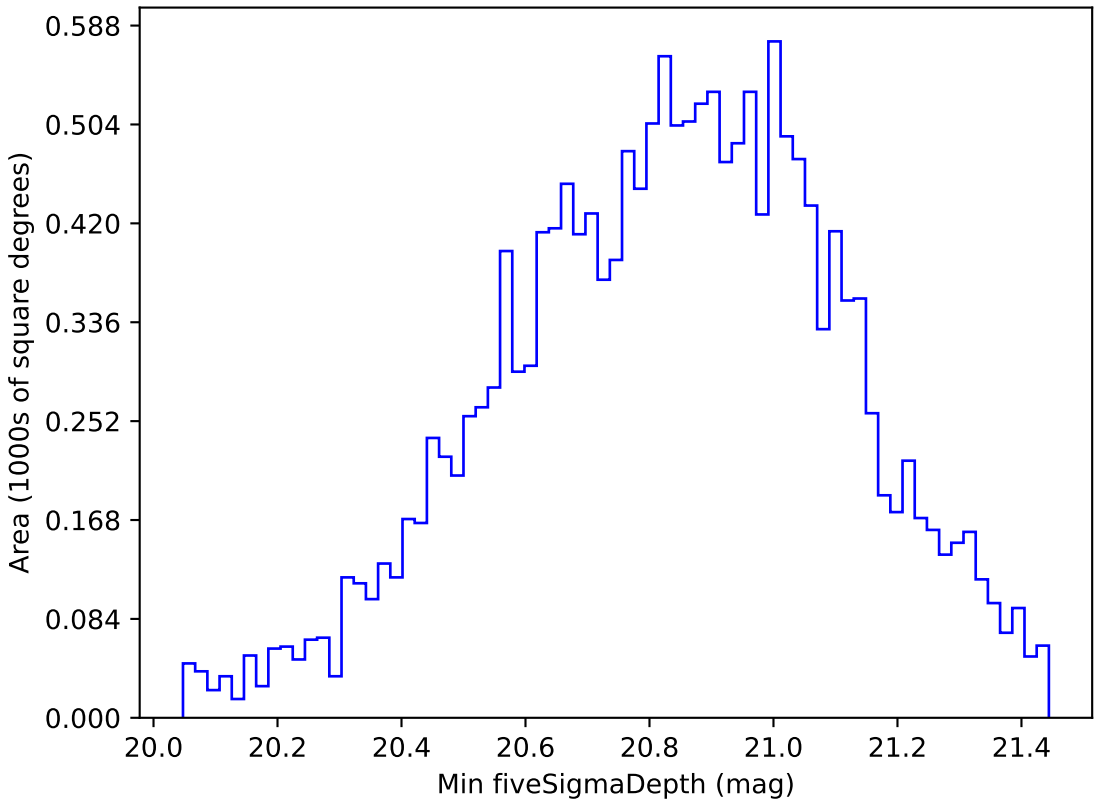
too_elab_r64_d2_giz_v3.4_10yrs WFD y band: Min fiveSigmaDepth
