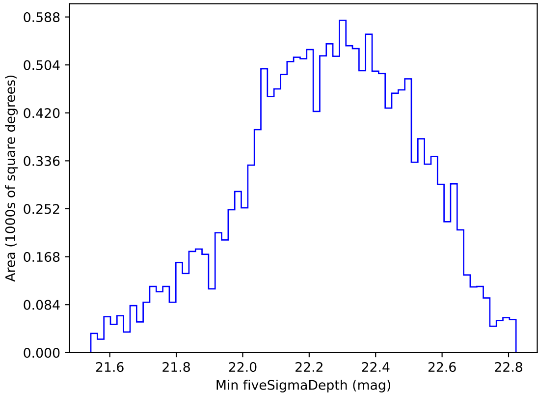
too_elab_r64_d2_giz_v3.4_10yrs WFD u band: Min fiveSigmaDepth
