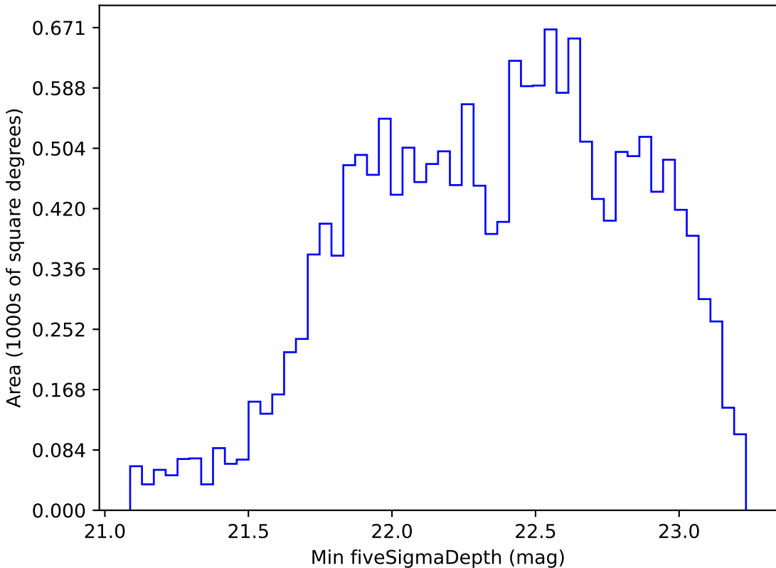
too_elab_r64_d2_giz_v3.4_10yrs WFD r band: Min fiveSigmaDepth
