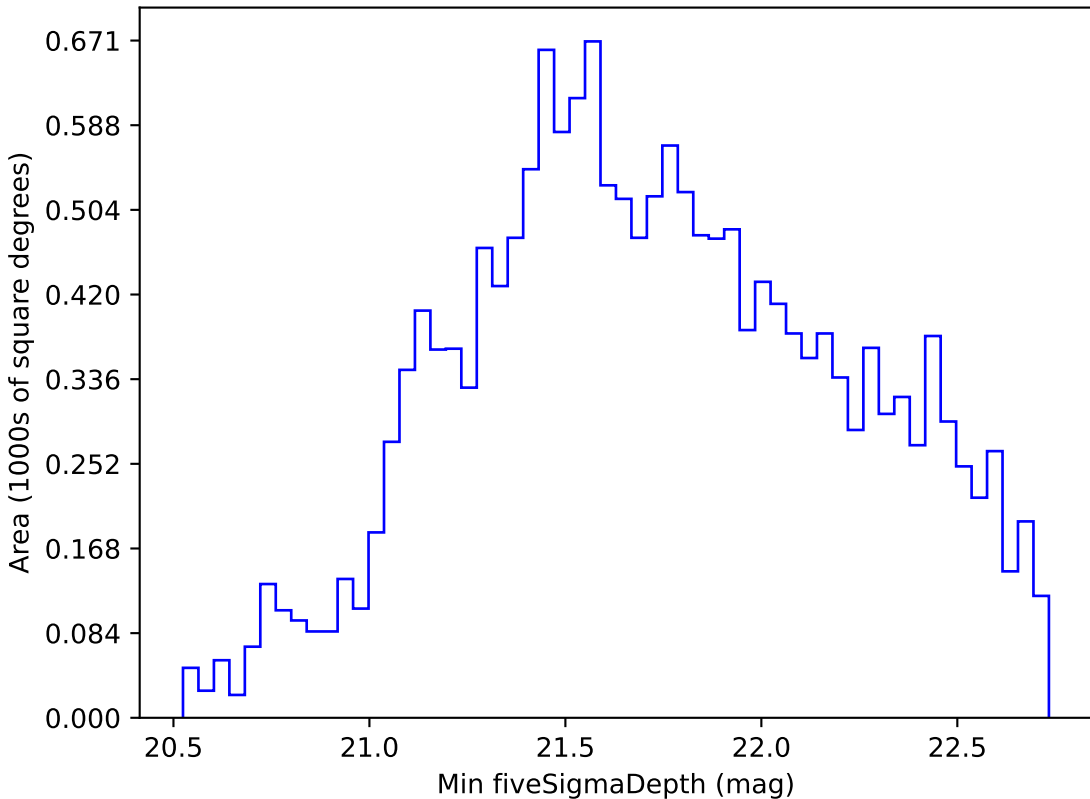
too_elab_r64_d2_giz_v3.4_10yrs WFD i band: Min fiveSigmaDepth
