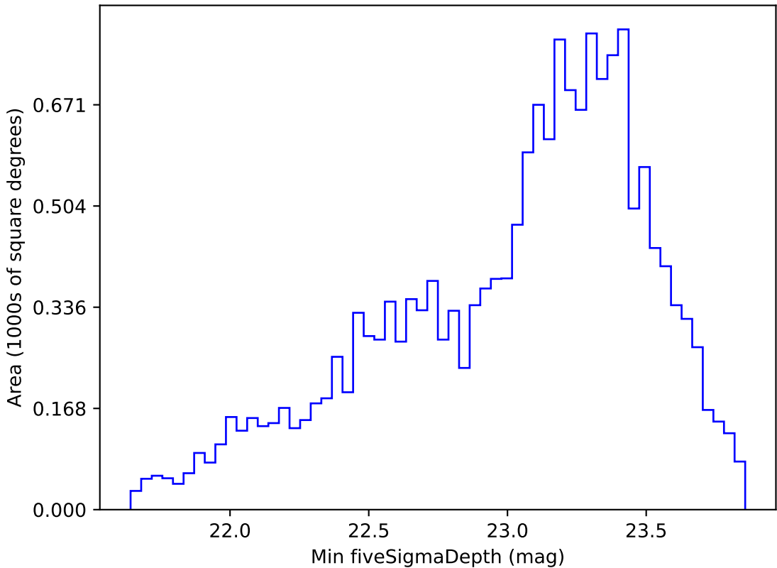
too_elab_r64_d2_giz_v3.4_10yrs WFD g band: Min fiveSigmaDepth
