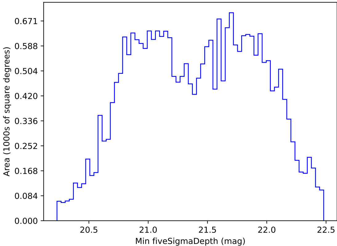
too_elab_r64_d2_giz_v3.4_10yrs All sky z band: Min fiveSigmaDepth
