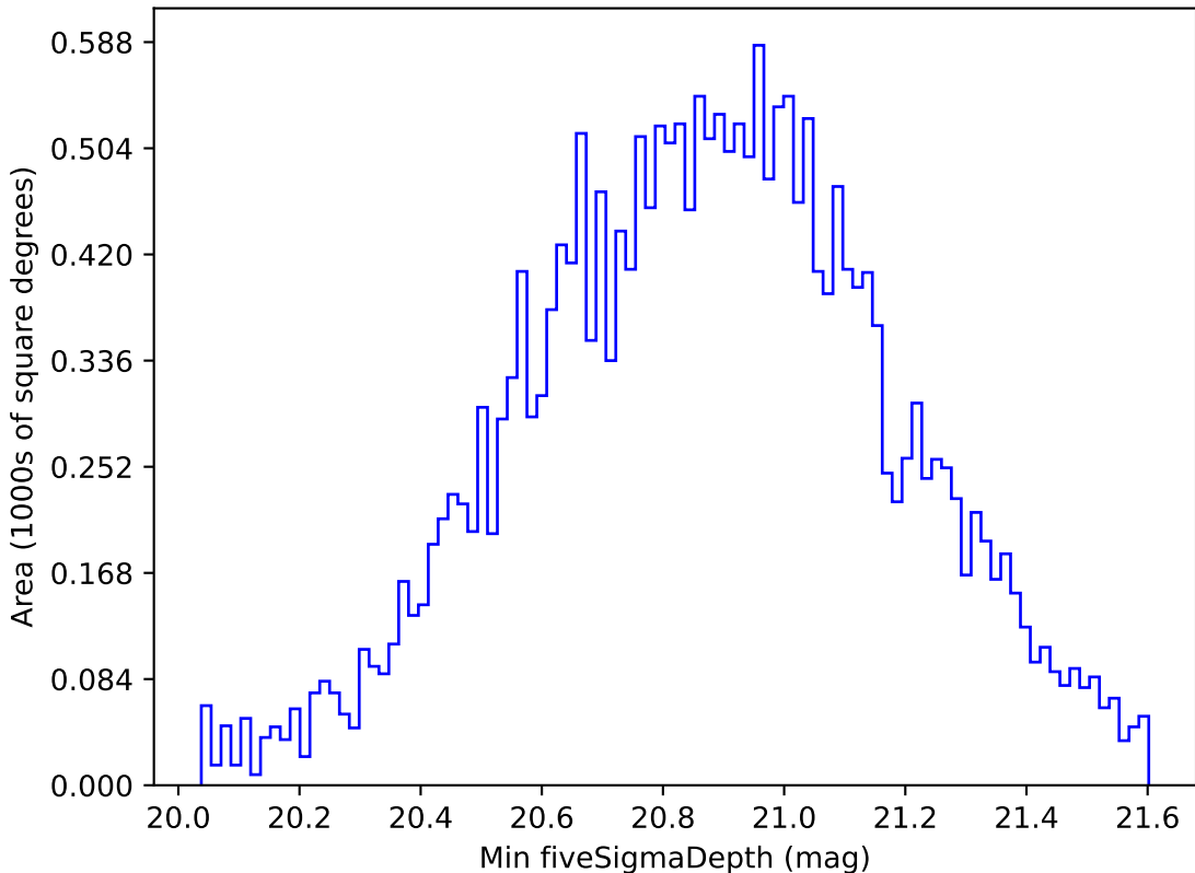
too_elab_r64_d2_giz_v3.4_10yrs All sky y band: Min fiveSigmaDepth
