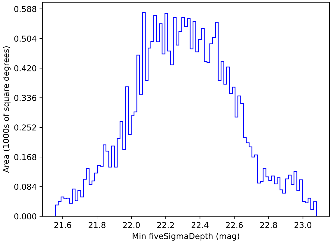
too_elab_r64_d2_giz_v3.4_10yrs All sky u band: Min fiveSigmaDepth
