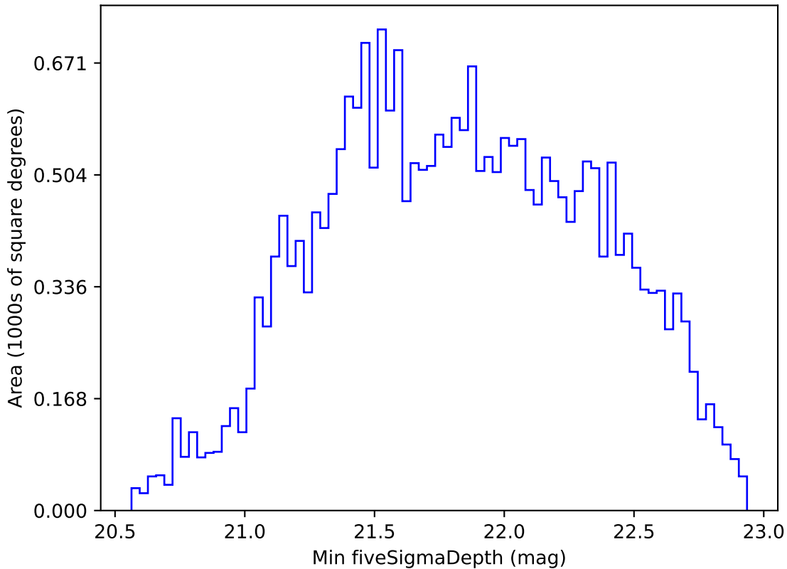
too_elab_r64_d2_giz_v3.4_10yrs All sky i band: Min fiveSigmaDepth
