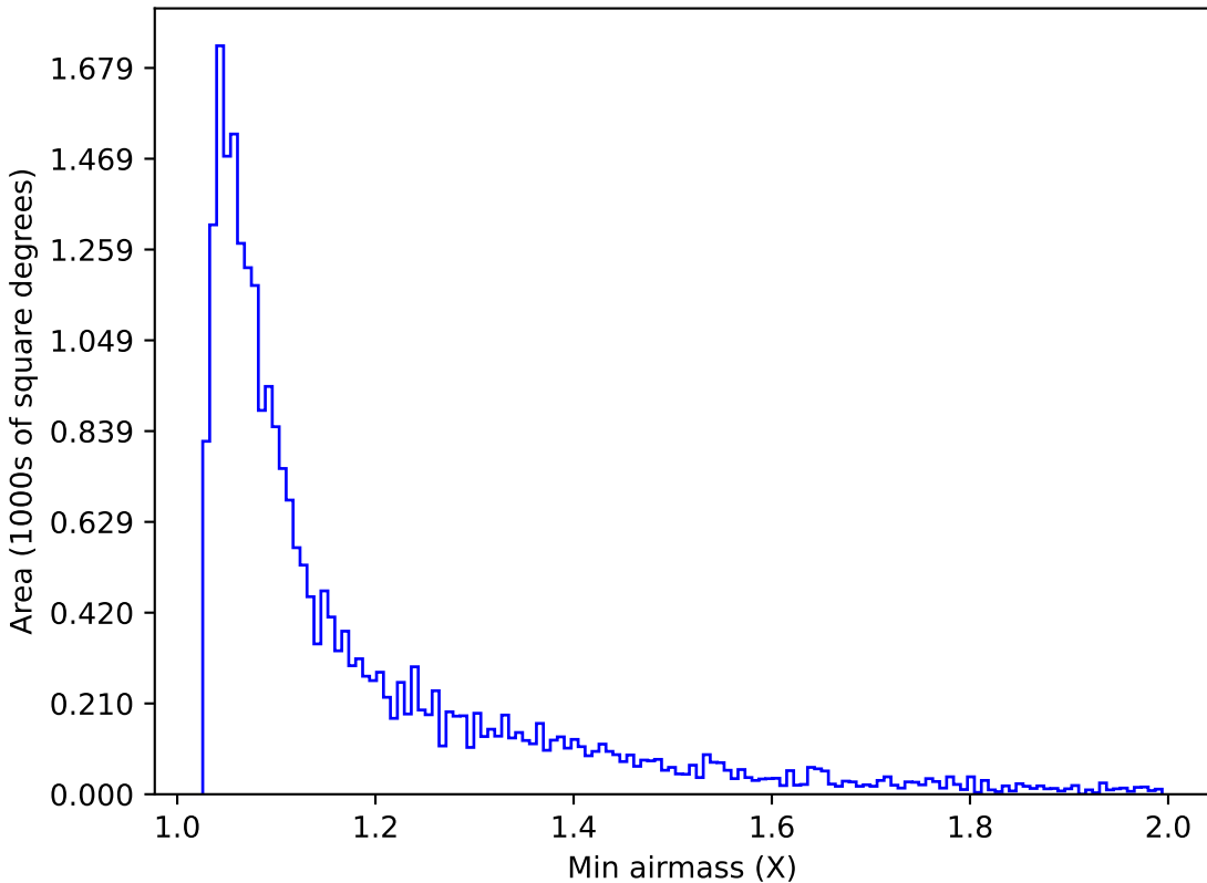
too_elab_r64_d2_giz_v3.4_10yrs Yr 1 g band: Min airmass
