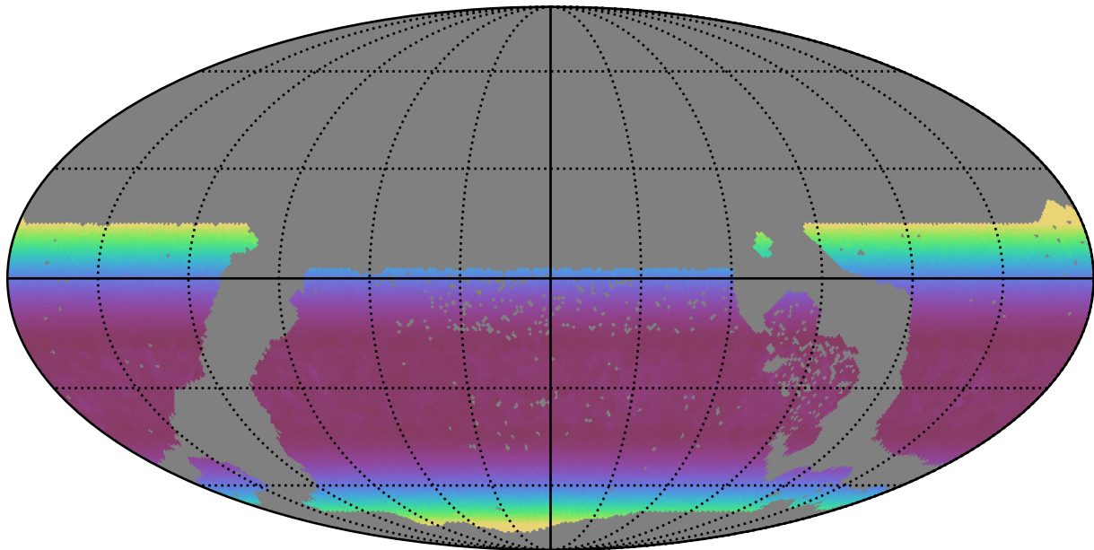
too_elab_r64_d2_giz_v3.4_10yrs WFD y band: Min airmass
