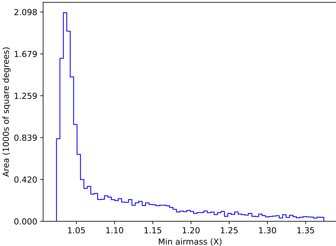
too_elab_r64_d2_giz_v3.4_10yrs WFD u band: Min airmass
