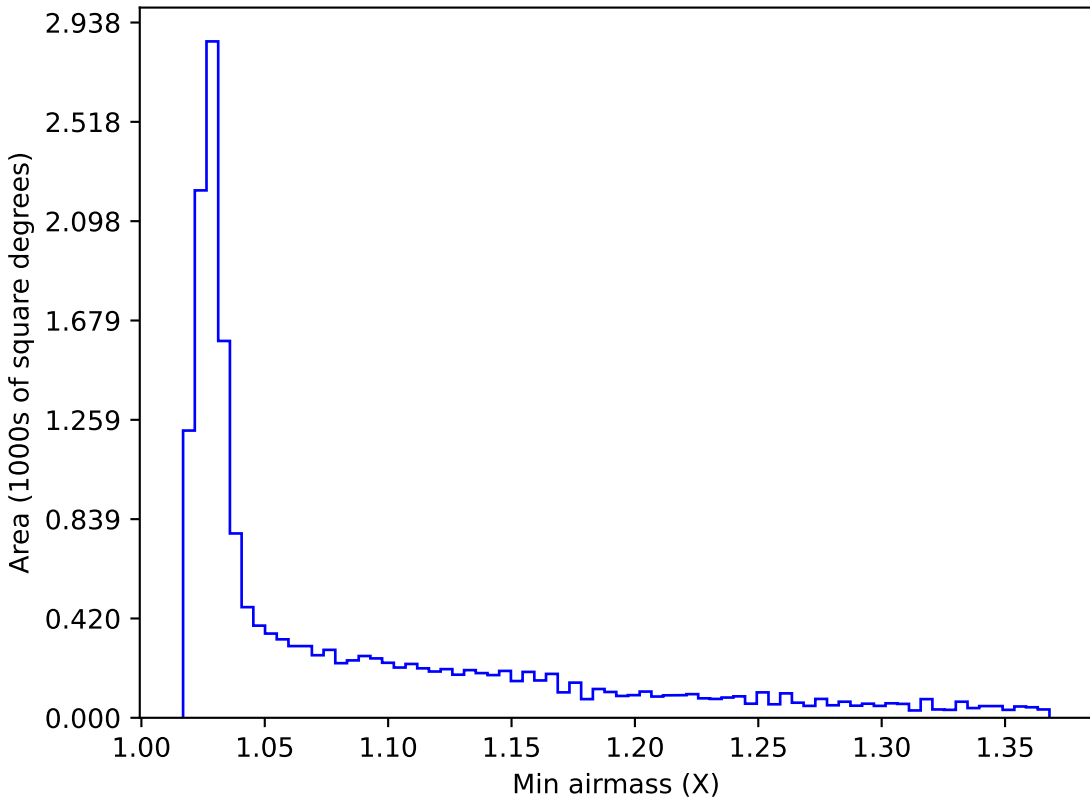
too_elab_r64_d2_giz_v3.4_10yrs WFD r band: Min airmass
