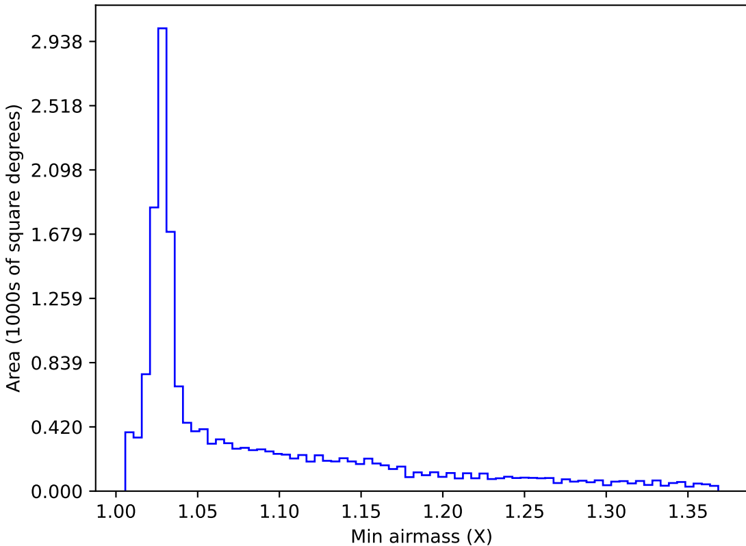
too_elab_r64_d2_giz_v3.4_10yrs WFD i band: Min airmass
