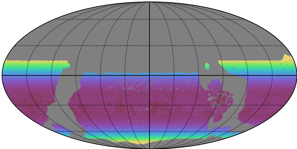
too_elab_r64_d2_giz_v3.4_10yrs WFD all bands: Min airmass
