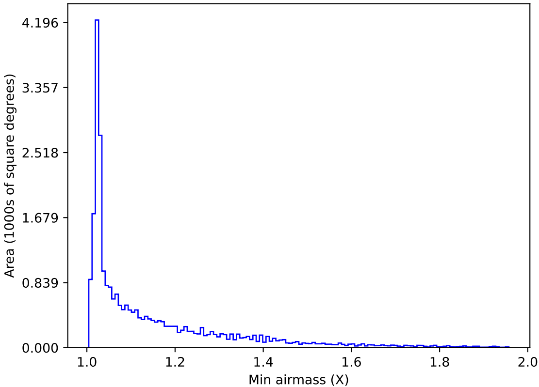
too_elab_r64_d2_giz_v3.4_10yrs All sky all bands: Min airmass
