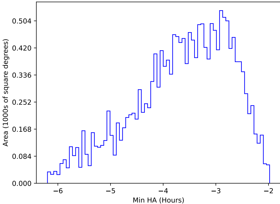
too_elab_r64_d2_giz_v3.4_10yrs WFD y band: Min HA
