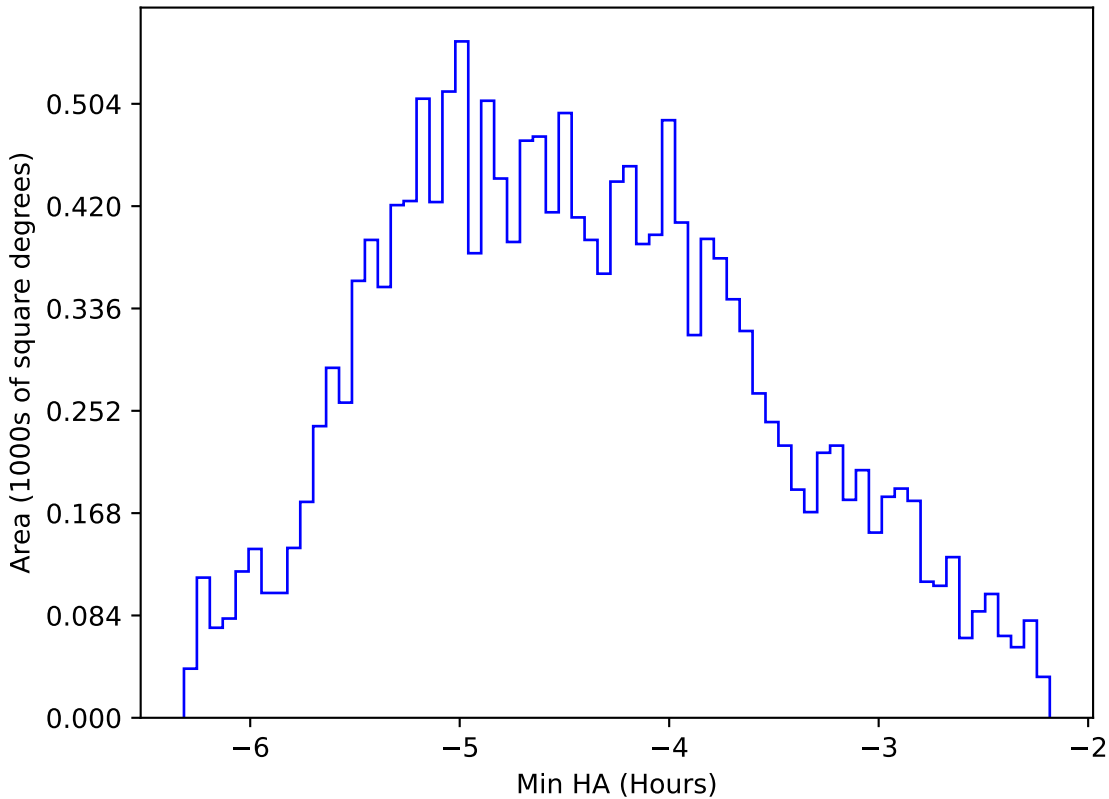
too_elab_r64_d2_giz_v3.4_10yrs WFD r band: Min HA
