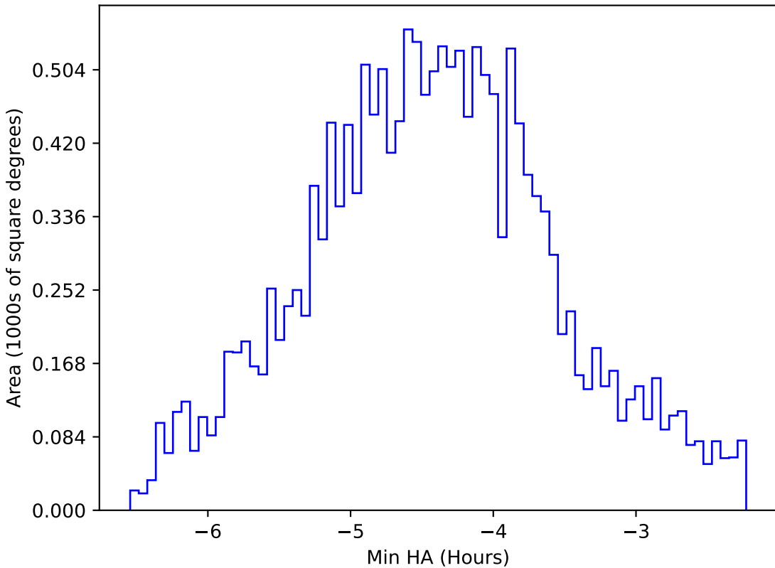
too_elab_r64_d2_giz_v3.4_10yrs WFD i band: Min HA
