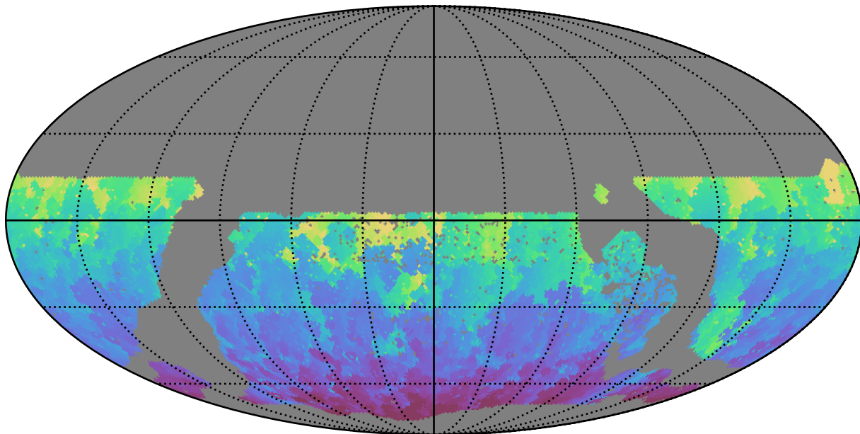
too_elab_r64_d2_giz_v3.4_10yrs WFD g band: Min HA
