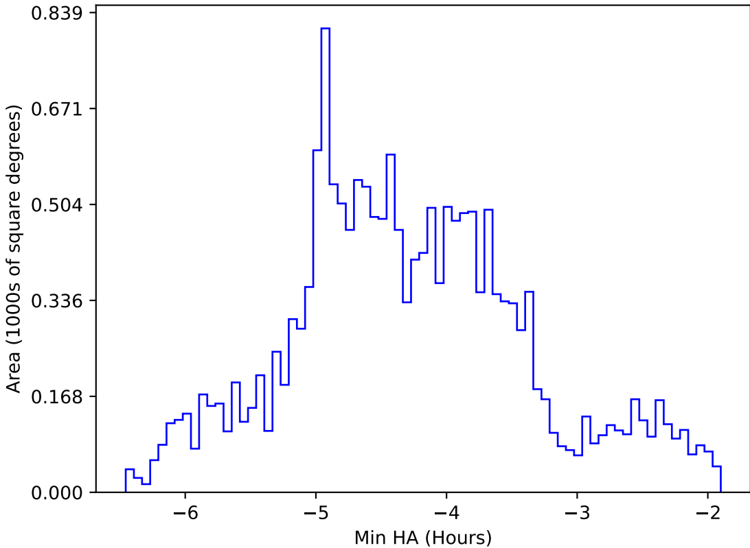
too_elab_r64_d2_giz_v3.4_10yrs WFD g band: Min HA
