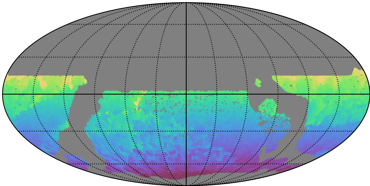
too_elab_r64_d2_giz_v3.4_10yrs WFD all bands: Min HA
