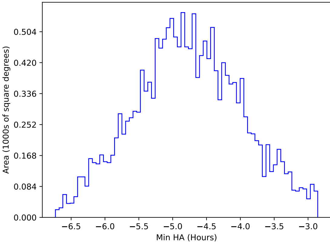
too_elab_r64_d2_giz_v3.4_10yrs WFD all bands: Min HA
