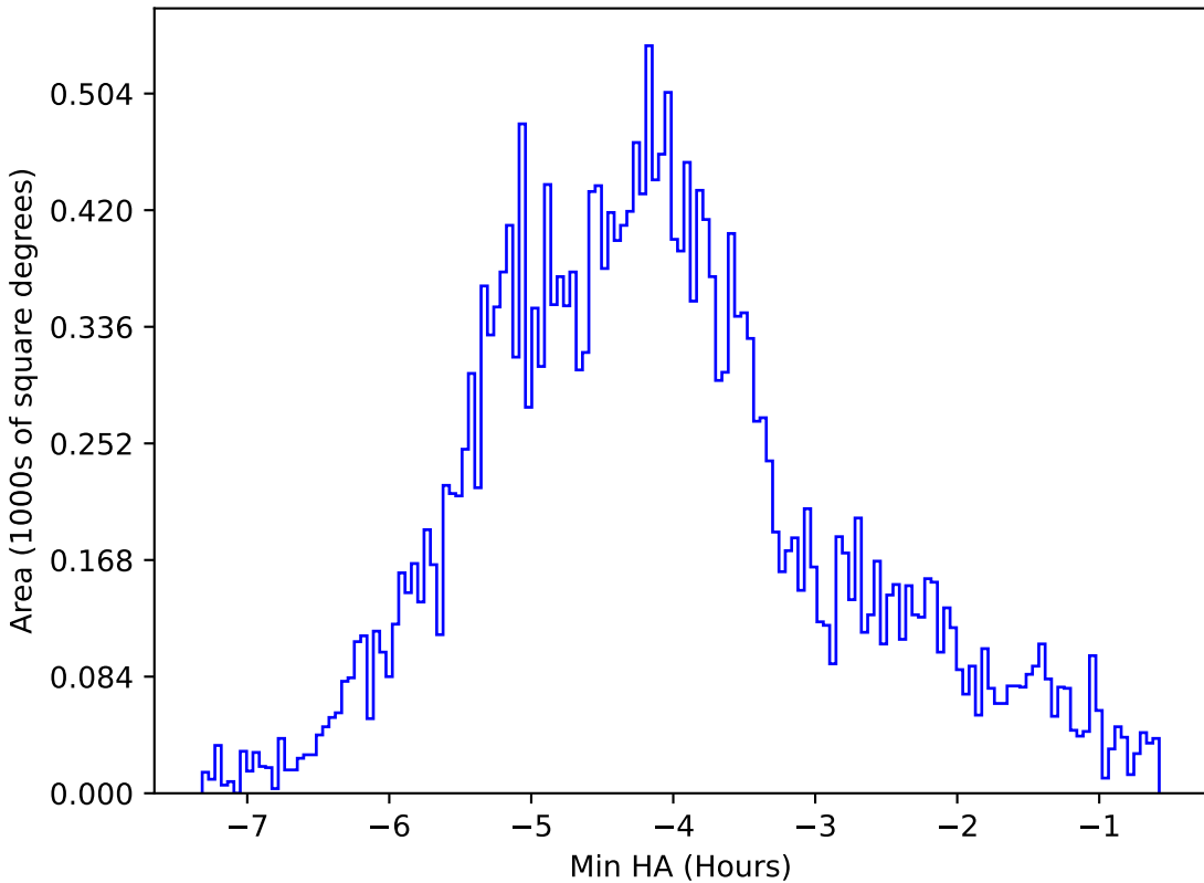
too_elab_r64_d2_giz_v3.4_10yrs All sky z band: Min HA
