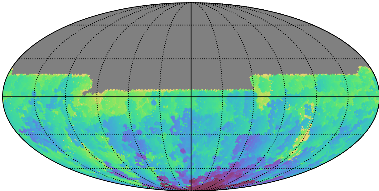
too_elab_r64_d2_giz_v3.4_10yrs All sky u band: Min HA
