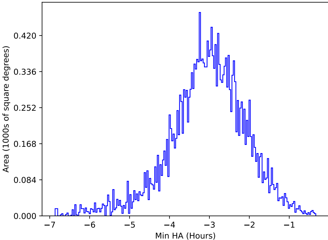
too_elab_r64_d2_giz_v3.4_10yrs All sky u band: Min HA
