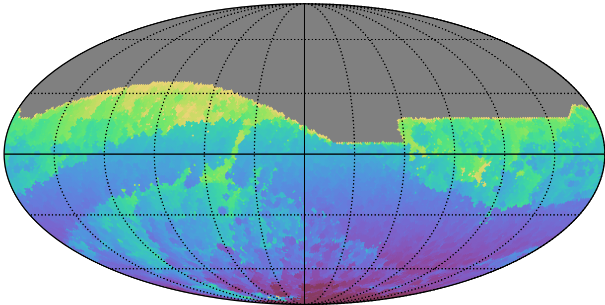
too_elab_r64_d2_giz_v3.4_10yrs All sky r band: Min HA
