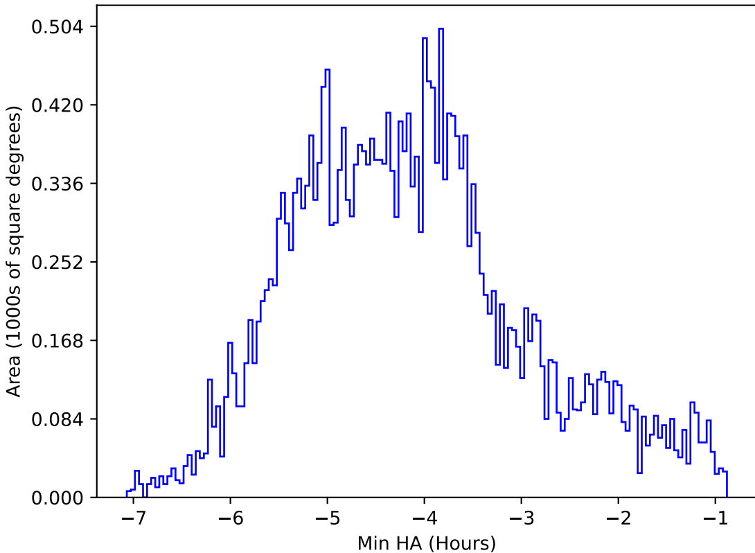
too_elab_r64_d2_giz_v3.4_10yrs All sky r band: Min HA
