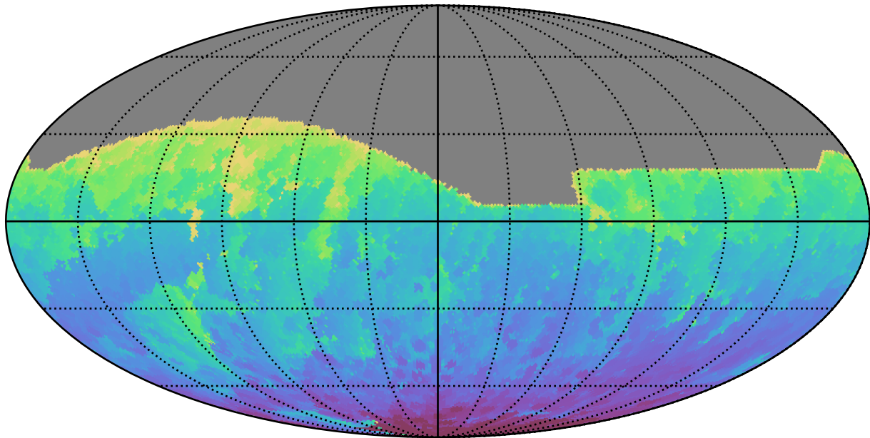
too_elab_r64_d2_giz_v3.4_10yrs All sky i band: Min HA
